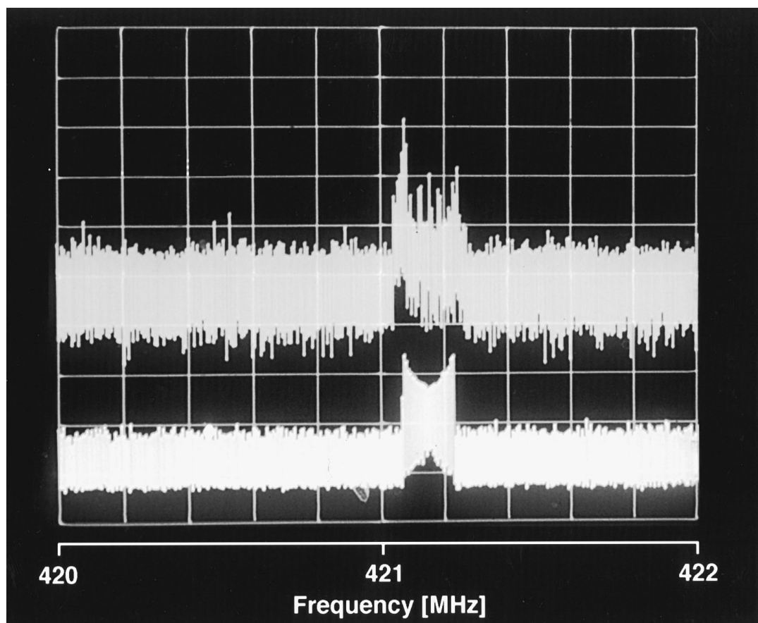
FIG. 1. (Top) A modulated ESR-STM signal detected only with a spectrum analyzer. It is observed under the conditions of field modulation described in the text. For comparison, an analogous frequency-modulated signal (bottom) from a frequency synthesizer is shown.
