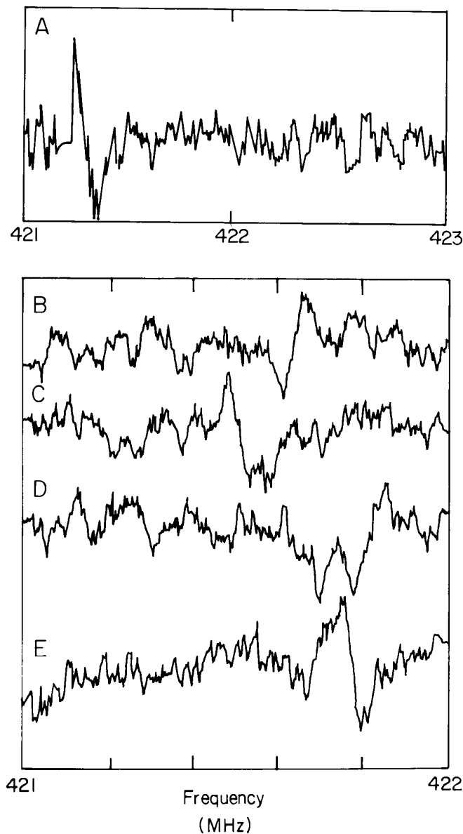
FIG. 3. Different ESR-STM spectra detected with a spectrum analyzer and a lock-in amplifier. The experimental modulation conditions are described in the text.
